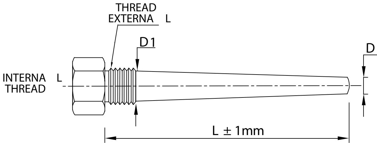
C.PO: Conical Steel Straight Tapered Solid drilled Pocket
