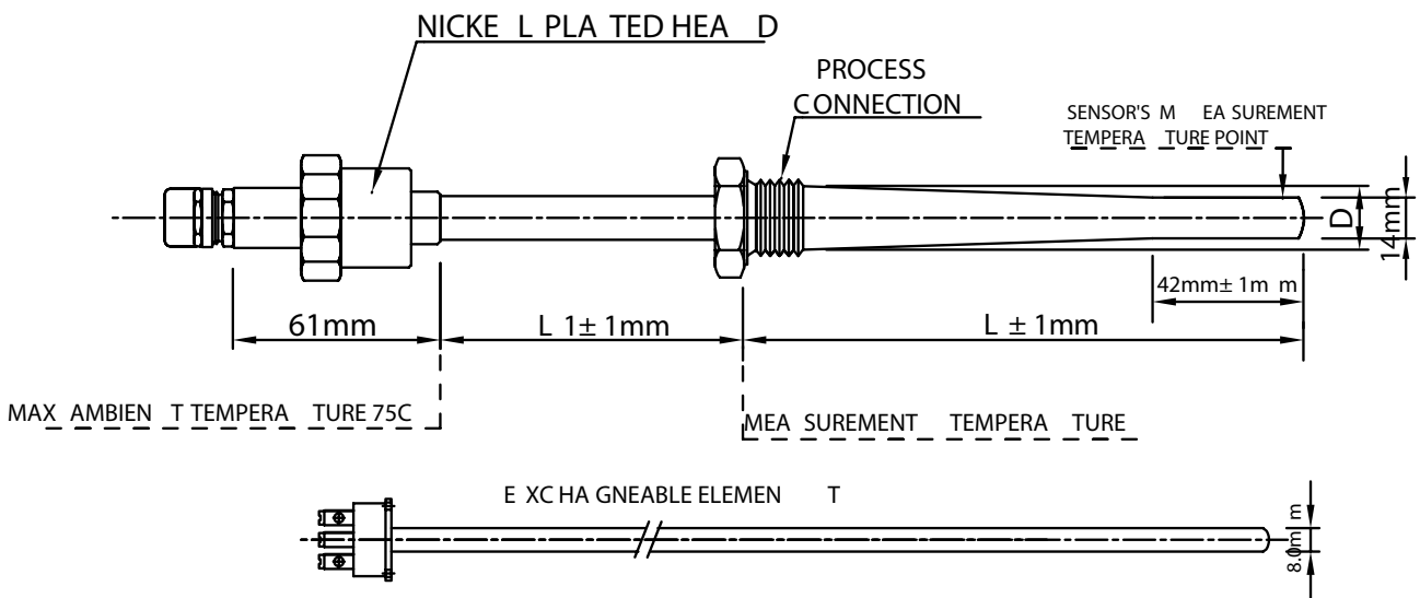
MTB51: Nickel Plated head/ Tapered / Protection sheath Solid Drilled
