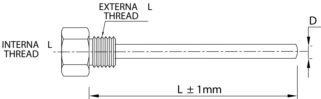
S.PO1: Stainless Steel Straight Pocket
